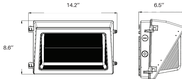
Variant 2: IK-WPKSC-01-S0120 (70W-85W-100W-120W)
