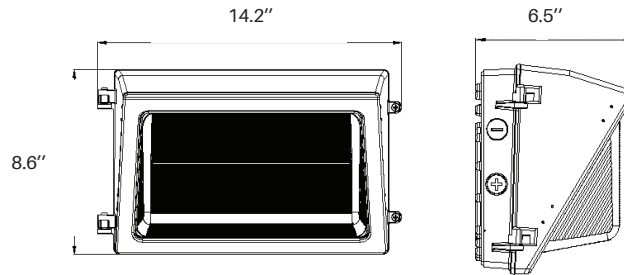
Variant 1: IK-WPKSC-01-S060 (30W-40W-50W-60W)
